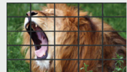
5 x 5 MATRIX
